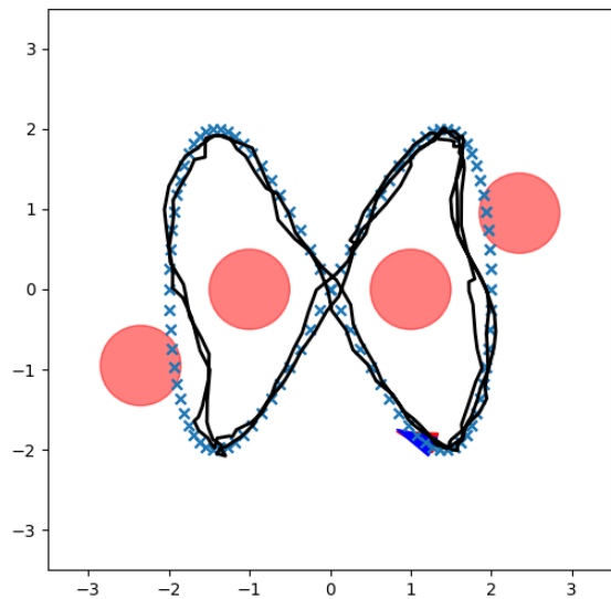
Fig. 1: Simulation of the unicycle car tracking a lemniscate trajectory in an environment with obstacles using Certainty Equivalent Control (CEC).
